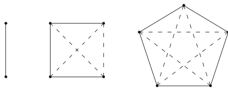
Figure 4. Simple cliques.
