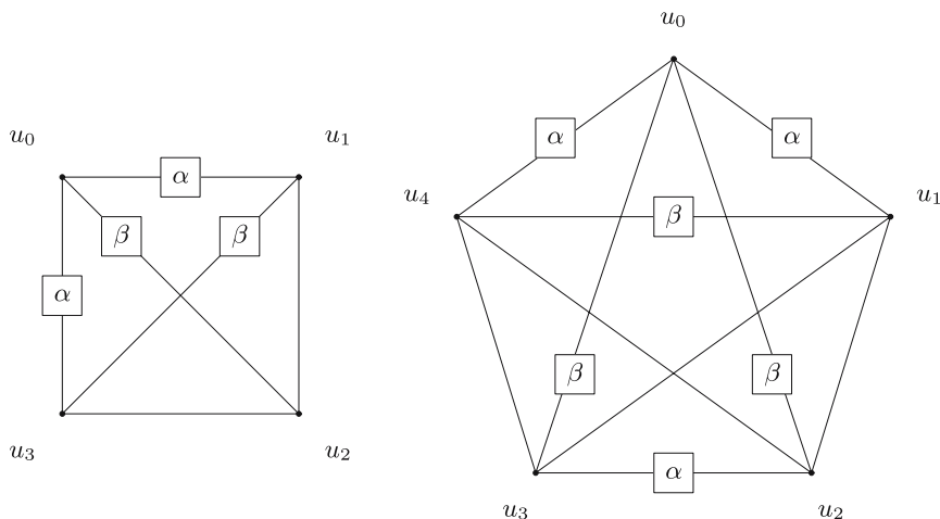
Figure 5. Proving Proposition 5.5.
