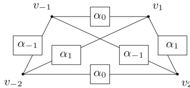
Figure 2. Construction of Proposition 3.7.
