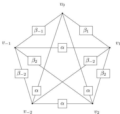
Figure 1. A colorful pentagon without colorful squares.
